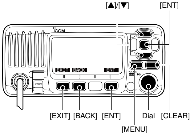
Menu lists
