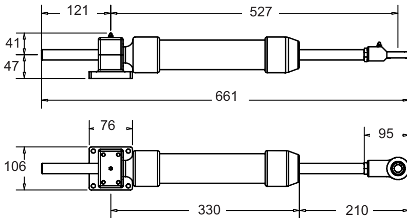
Model 210 Cylinder dimensions
