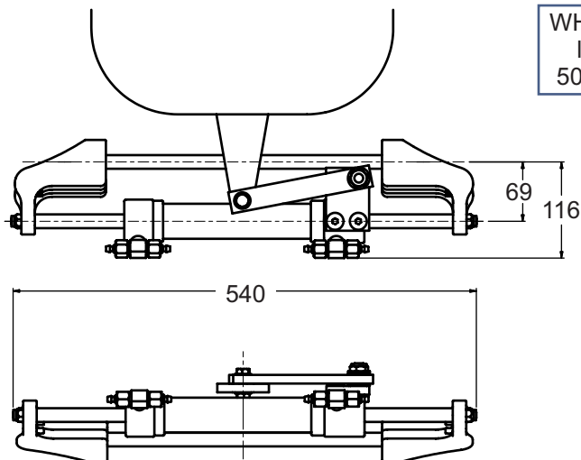
Model 511BH Cylinder dimensions
