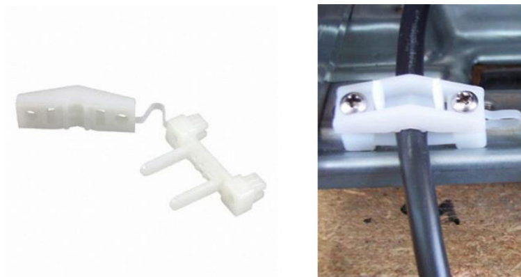
Figure 13: Detail of cable double fastening
