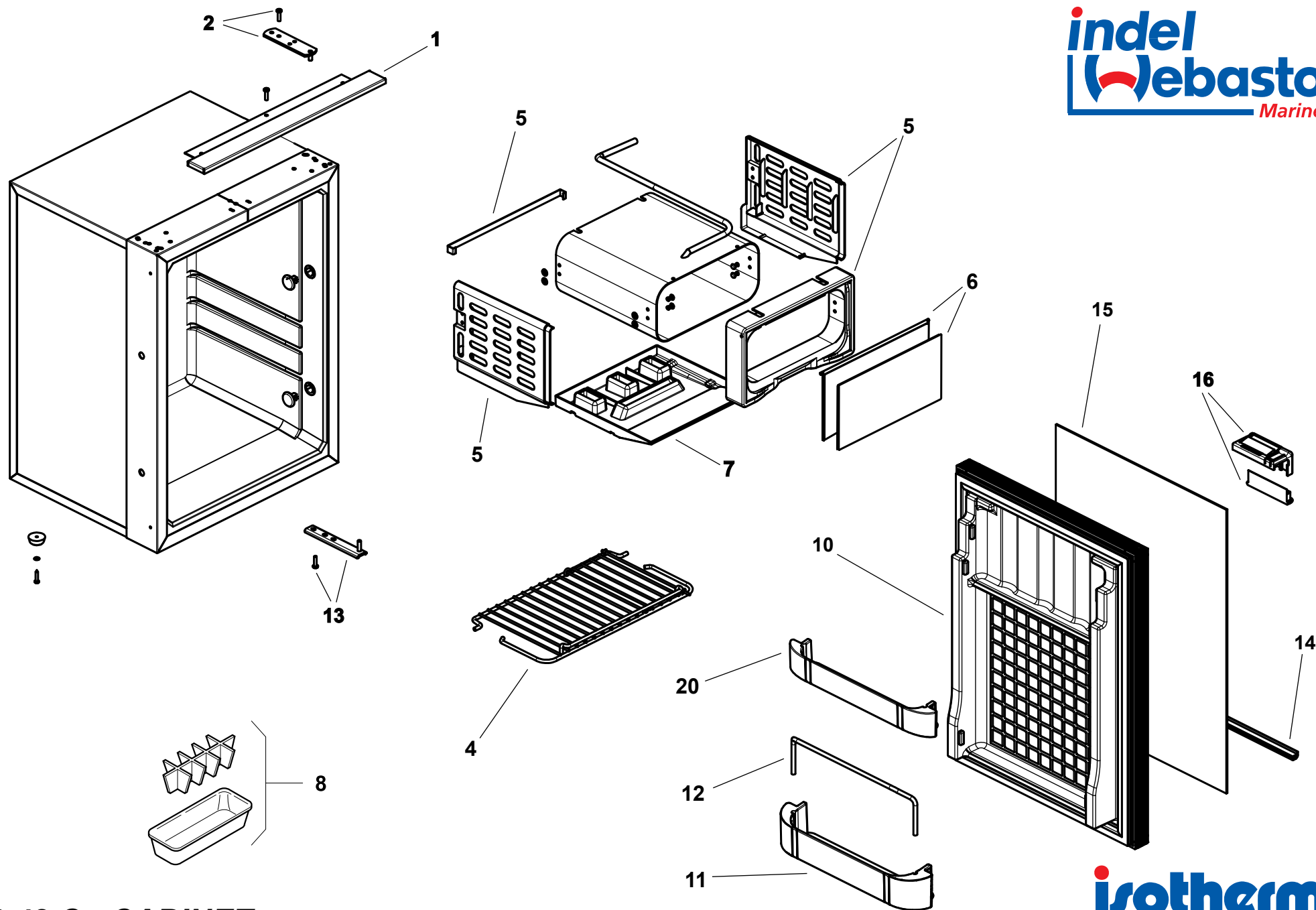
CR 42 C - CABINET
