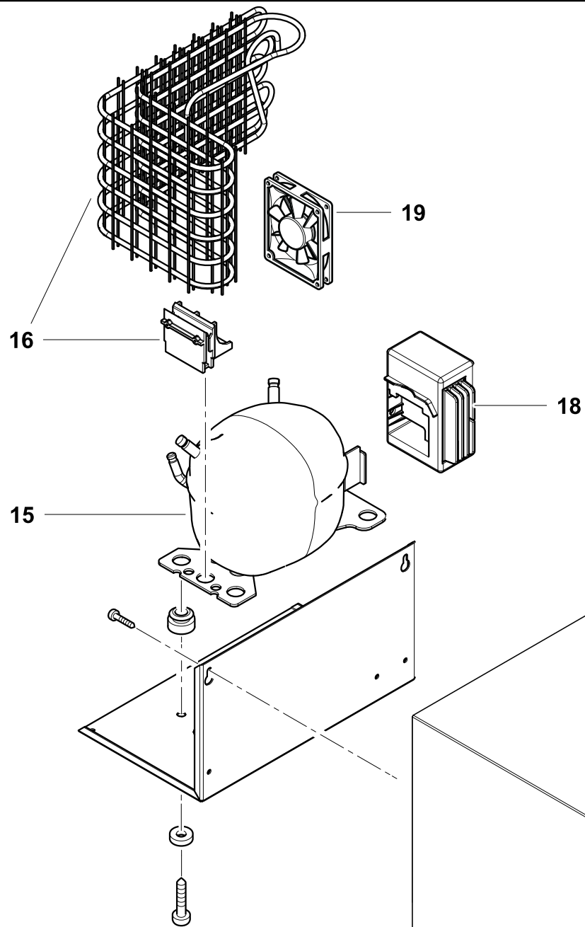
CR 40 - COOLING UNIT
